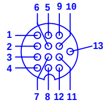
13 Pins female connector
